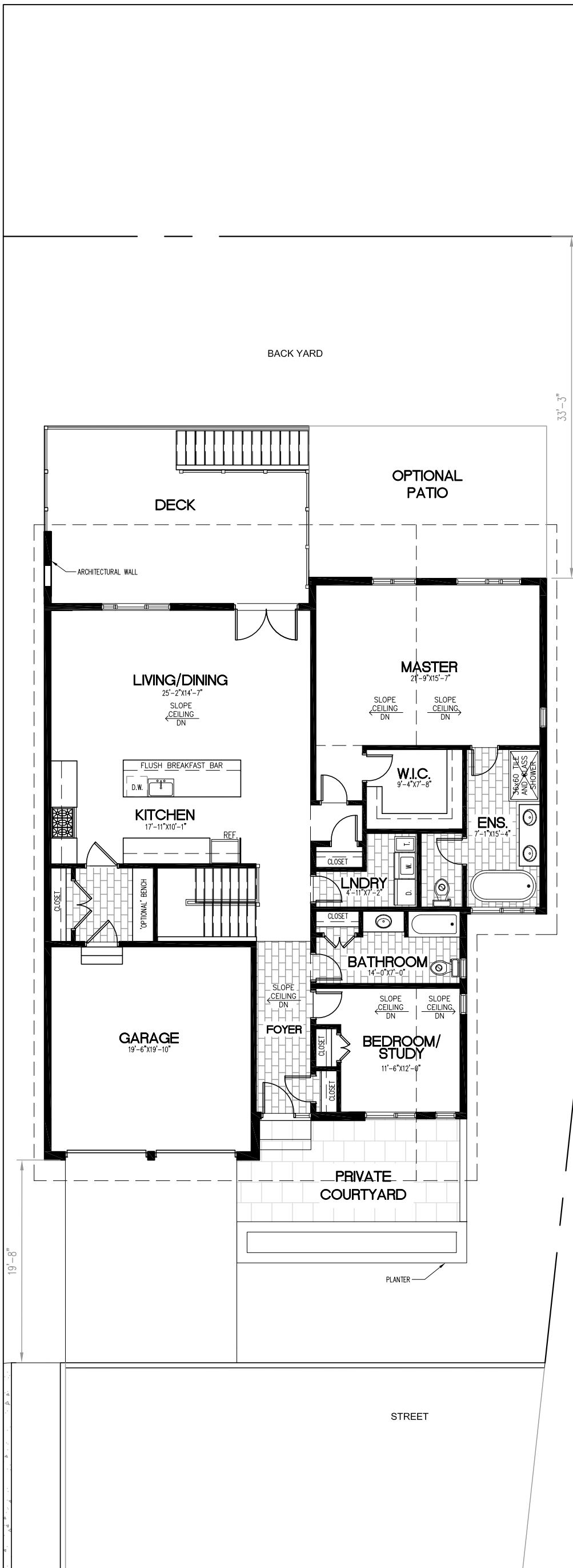
UNIT 30 2013 sqft MAIN FLOOR PLAN
